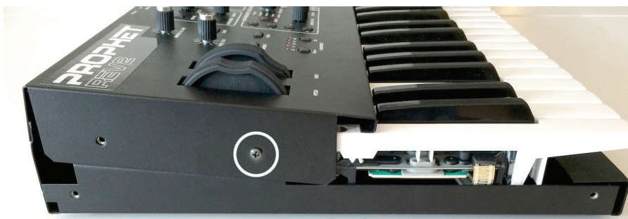
Remove the single screw on the both the right and left sides of the metal case
